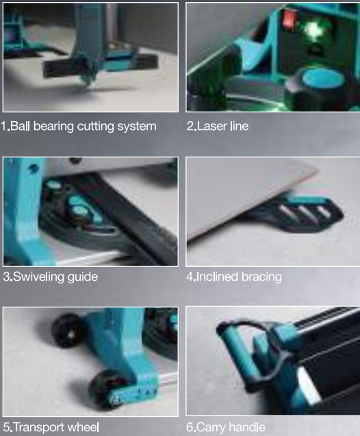
5.Transport wheel
