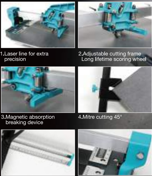
1.Laser line for extra precision 2.Adjustable cutting frame Long lifetime scoring wheel 3.Magnetic absorption breaking device 4.Mitre cutting 45° 5.Extension bars for 1.5M mitre cutting 6.Solid rail system
