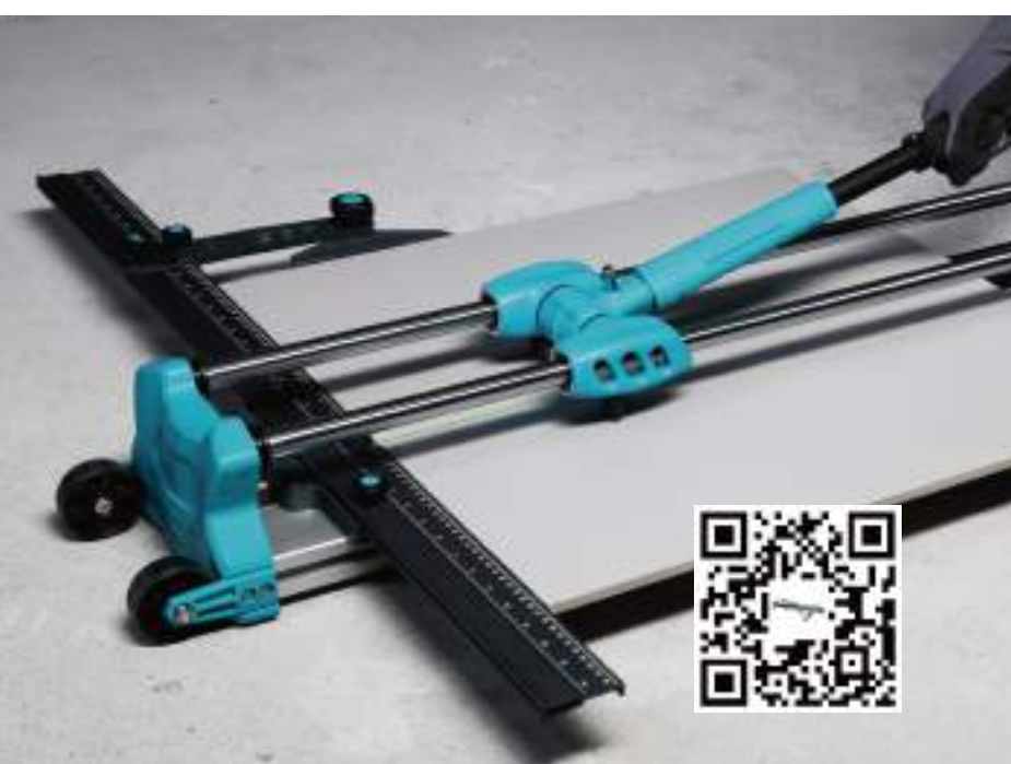
4.Adjustable measurement guide and side ruler
