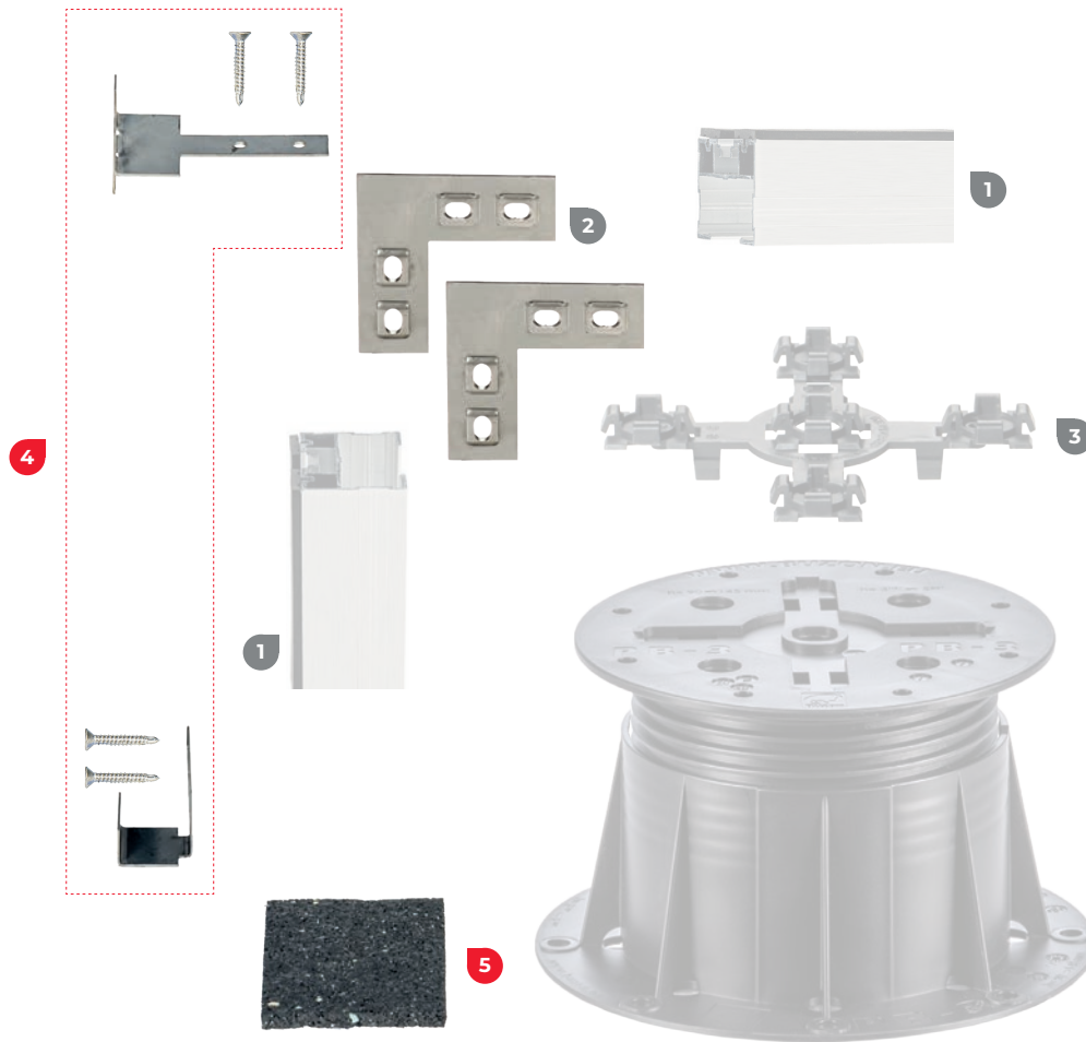
PIEDESTAL PB
