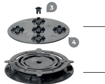
PIEDESTAL PB
